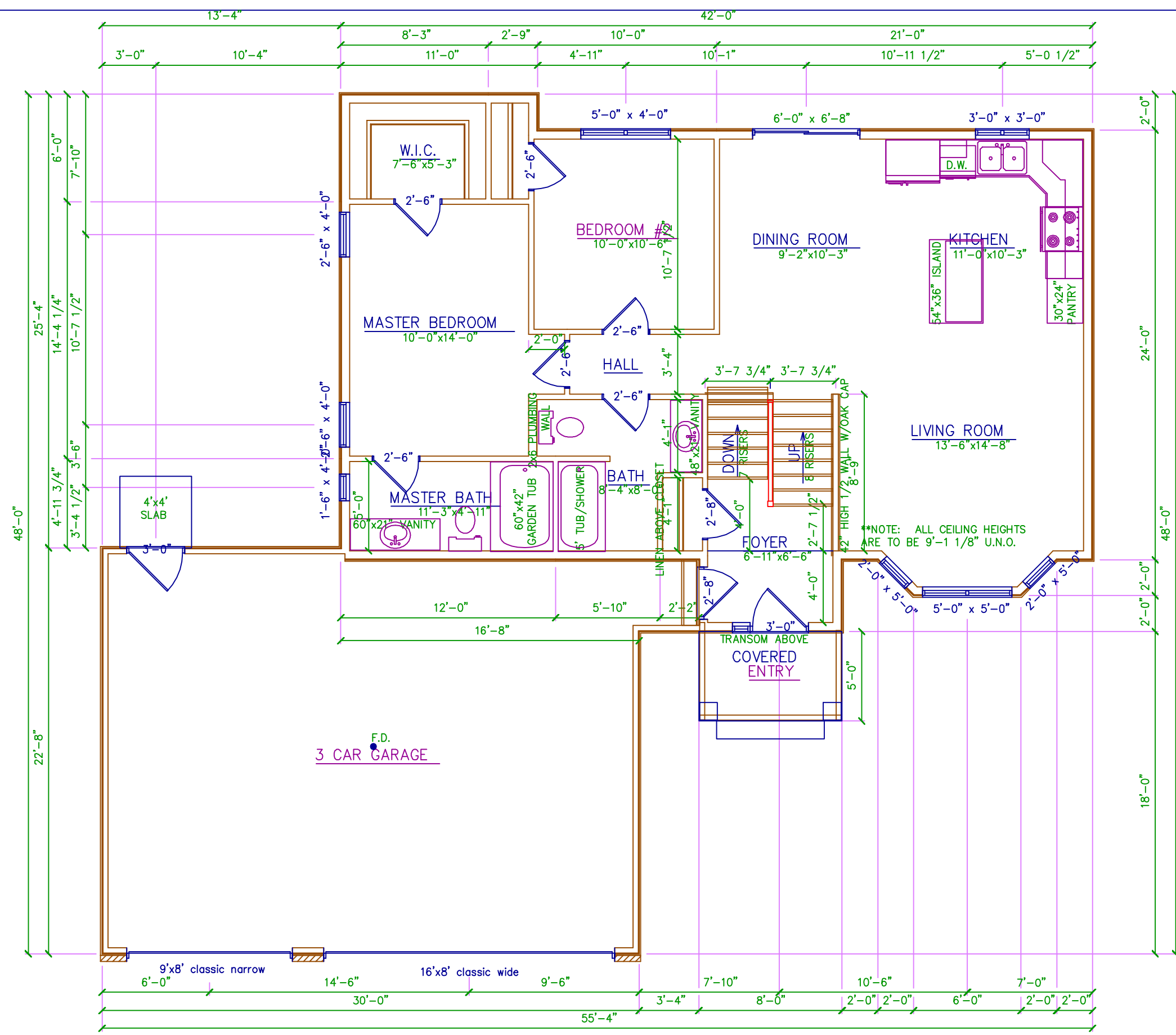
1ST FLOOR PLAN SCALE: 1/4" = 1'-0"
