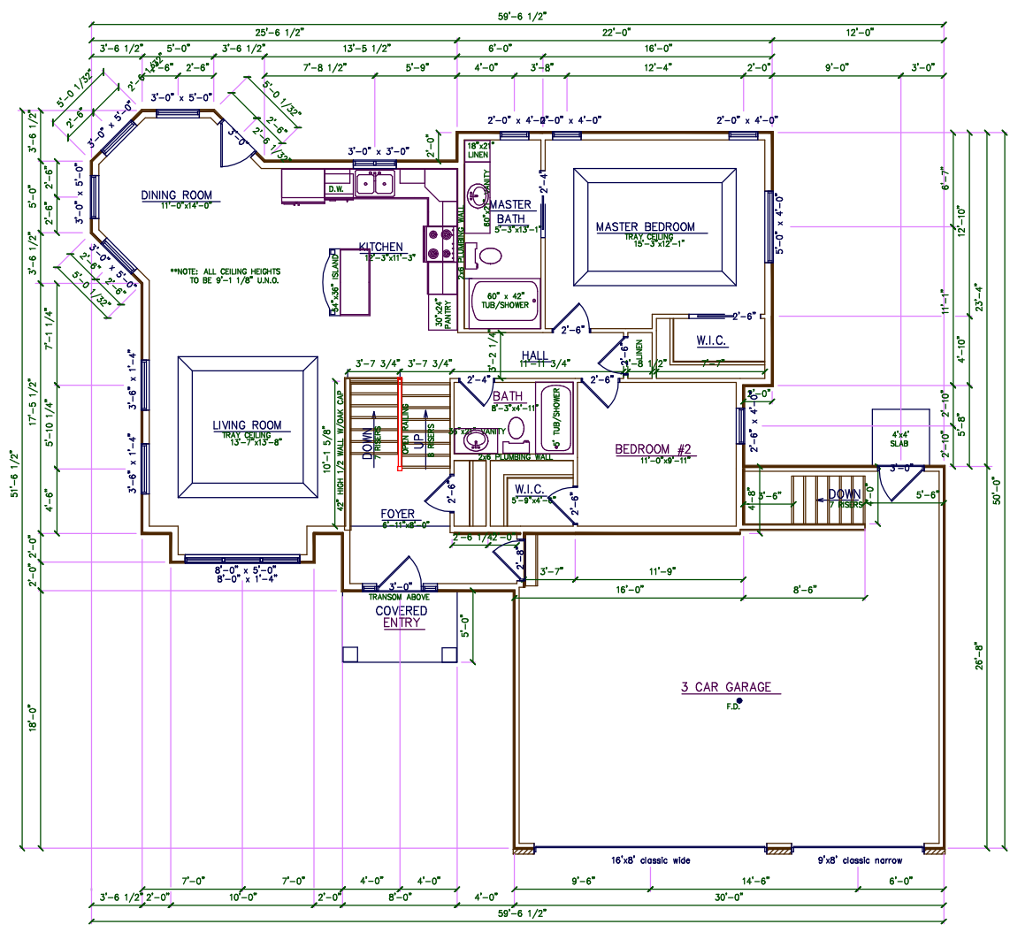
FLOOR PLAN SCALE: 1/4" = 1'-0"
