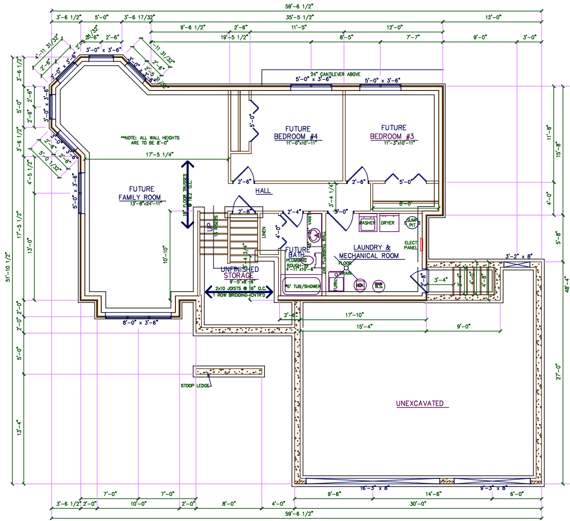
BASEMENT PLAN
