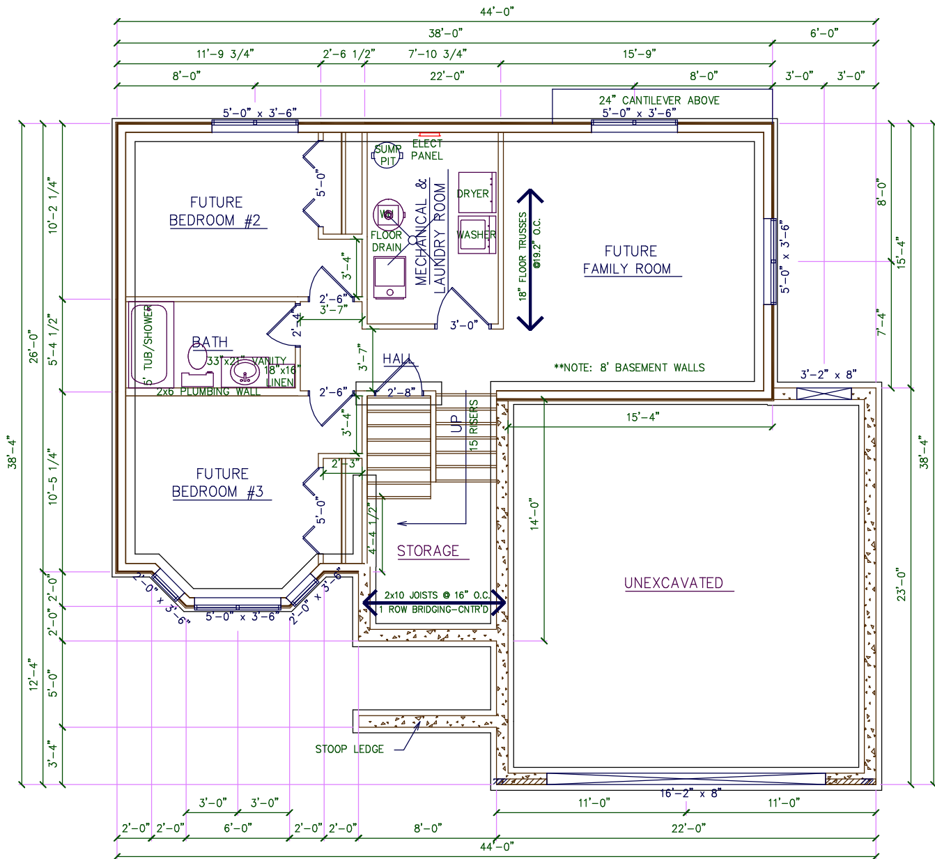
BASEMENT PLAN
