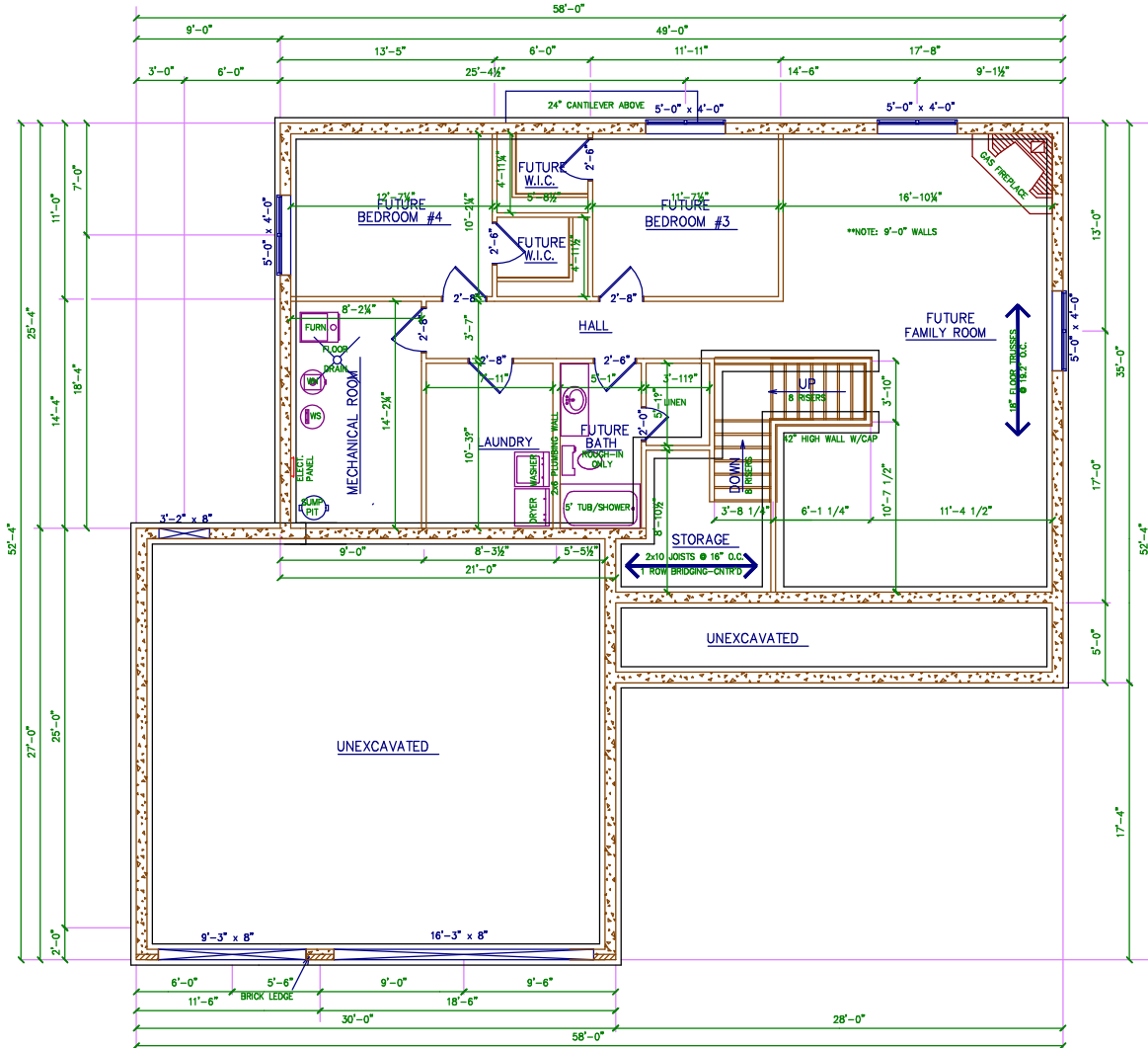
BASEMENT PLAN SCALE: 1/4" = 1'-0"
