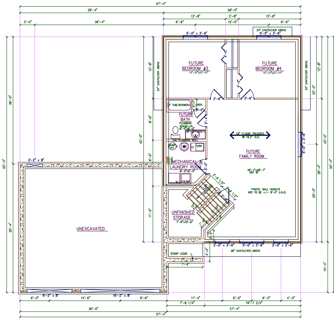
BASEMENT PLAN SCALE: 1/4" = 1'-0"
