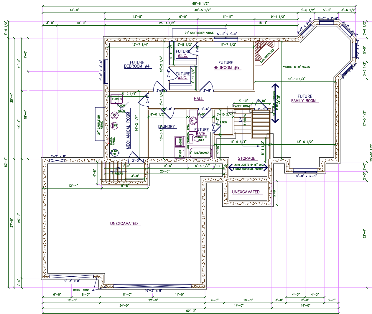
BASEMENT PLAN SCALE: 1/4" = 1'-0"
